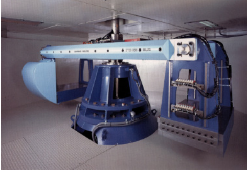
Figure 2. Centrifuge
