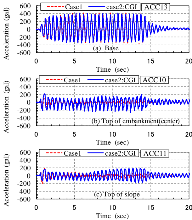
Figure 6. Response acceleration of base and embankment
