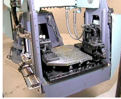
Figure 3. Shaking table
