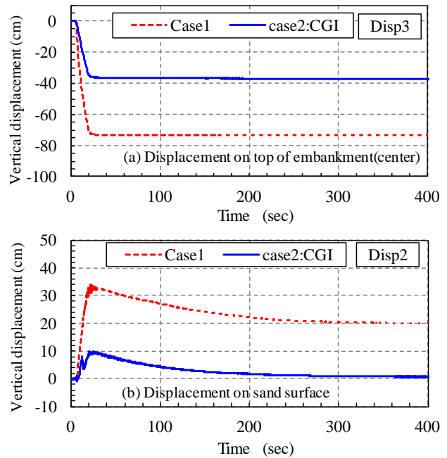
Figure 9. Vertical displacement
