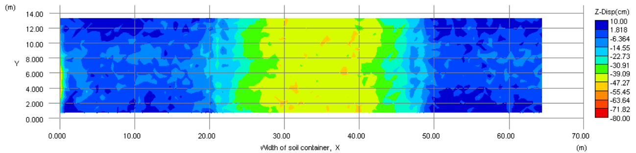
(b) Vertical displacement distribution of Case2 (CGI method)
