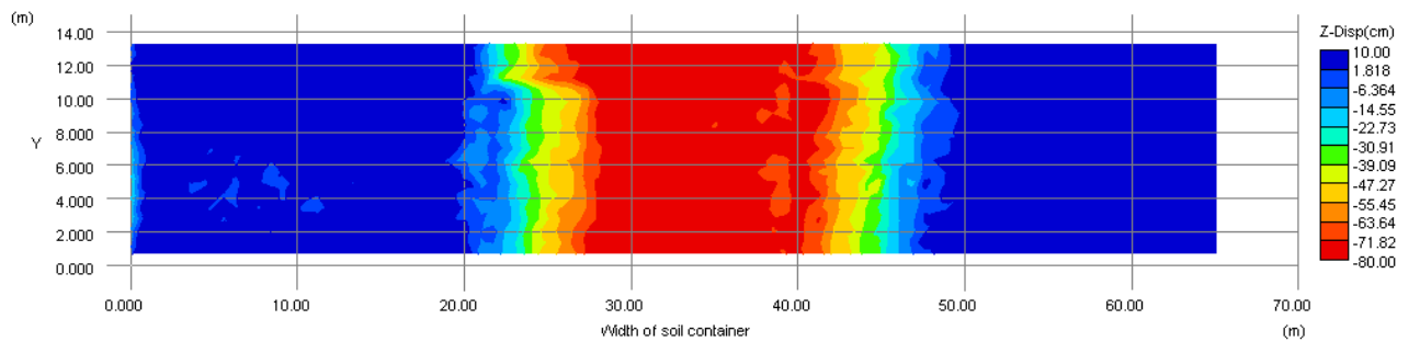
(a) Vertical displacement distribution of Case1 (without countermeasure)
