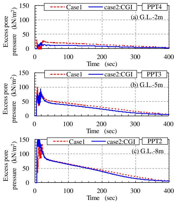
Figure 8. Excess pore pressure in sand layer (under embankment)
