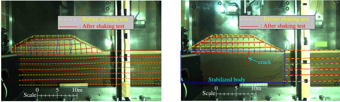
(a) Case1: without countermeasure
