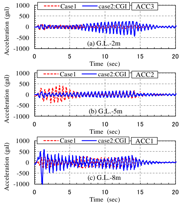
Figure 7. Response acceleration of sand layer (liquefaction layer)
