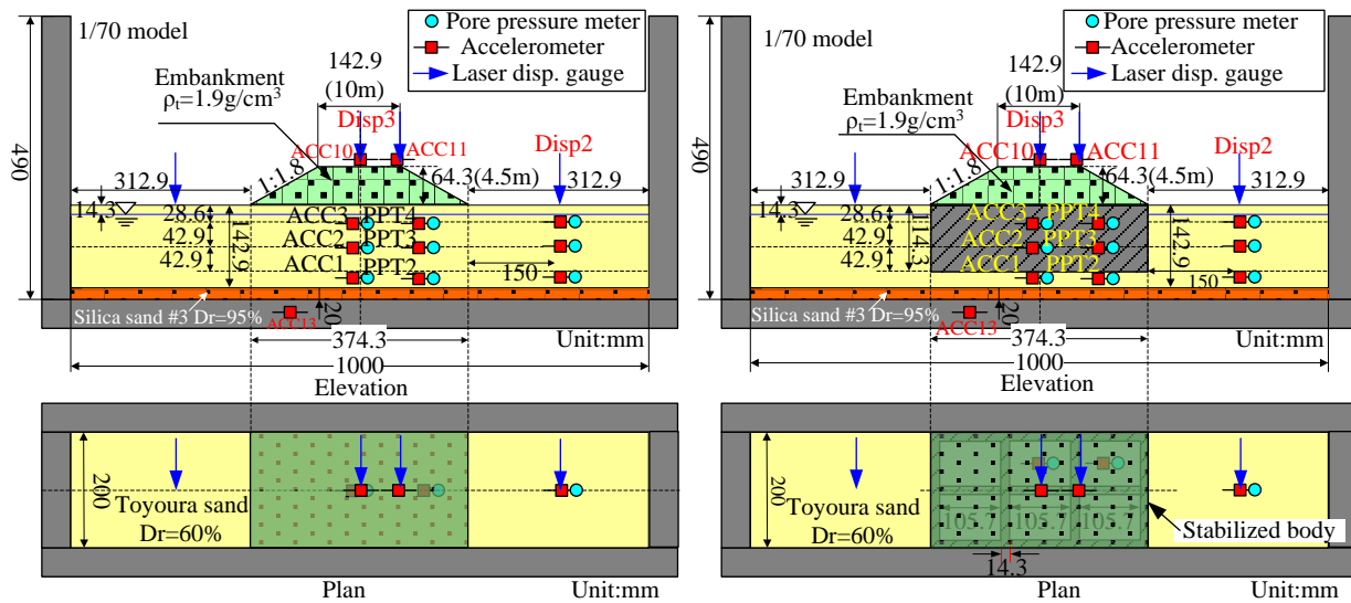
(a) Without Countermeasure (Case 1)
