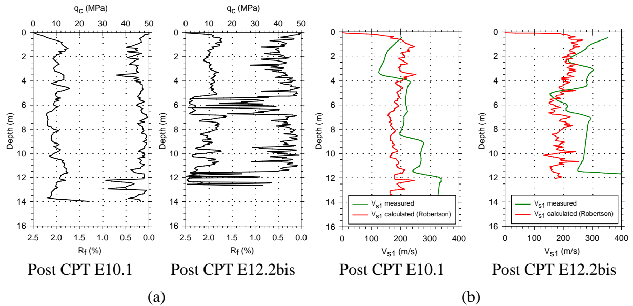
Figure 4. (a) Comparisons Post-CPT / normalized shear wave propagation velocities V_{s1} (b) Comparisons V_{s1} measured / V_{s1} calculated
